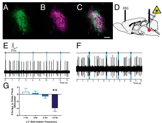
Fig. 1. Selective optogenetic control of LC-NE neurons at subarousal levels. LC neurons identified with TH staining (A, green) were transduced to selectively express ChR2-mCherry (B, magenta) at high levels (C, merge). (Scale bar: 100 \mu\text{m} .) (D) Schematic of glass pipette optrode and PFC EEG recording configurations. (E) Pulses of blue light elicited reliable short-latency single-action potentials from LC neurons in vivo (Inset, LC unit waveform) at 1 Hz up to 15 Hz. (F) Short trains of 15-Hz phasic light pulses evoked phasic excitation of LC neurons, followed by a postactivation inhibition pattern comparable to innate phasic LC responses to salient stimuli. (G) Increases in tonic LC stimulation dose-dependently increased arousal, as seen by a reduction in \delta -dominant EEG recordings at frequencies >5 Hz. **P < 0.01 relative to baseline arousal.
